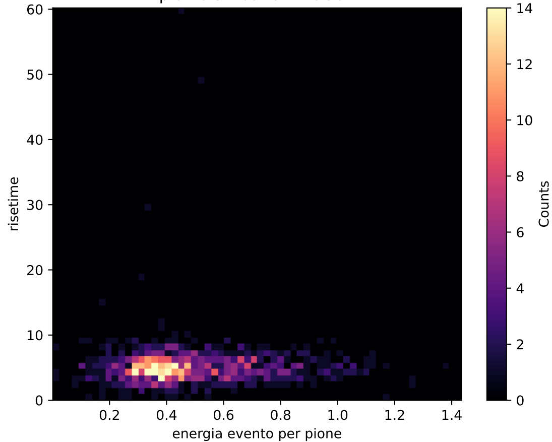
pion distribution 1.0GeV
