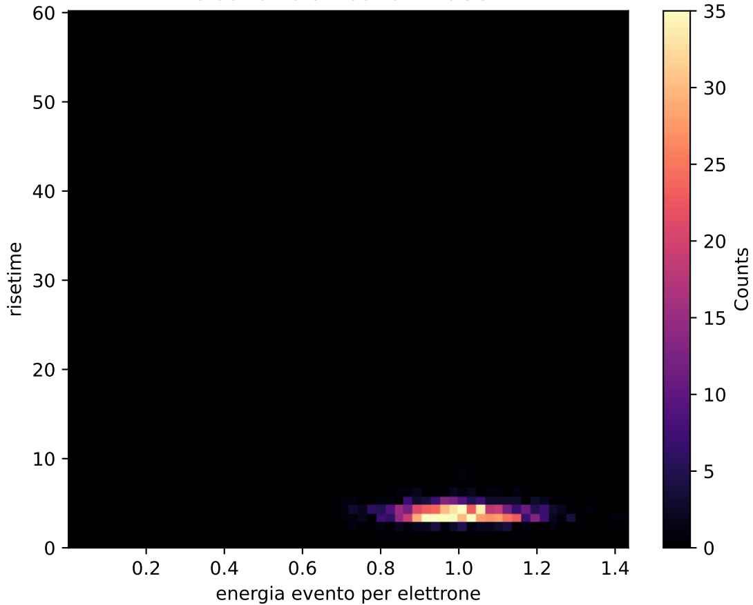
electron distribution 1.0GeV
